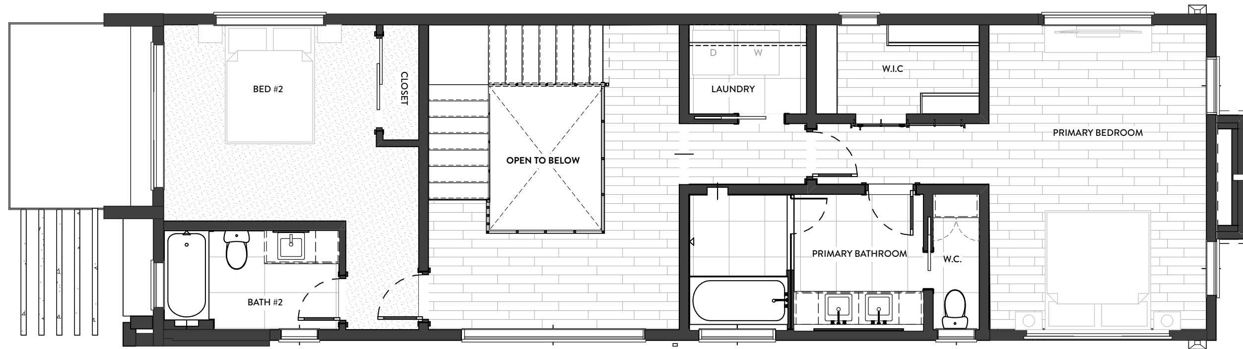
1 SECOND FLOOR 3/16" = 1'-0"
