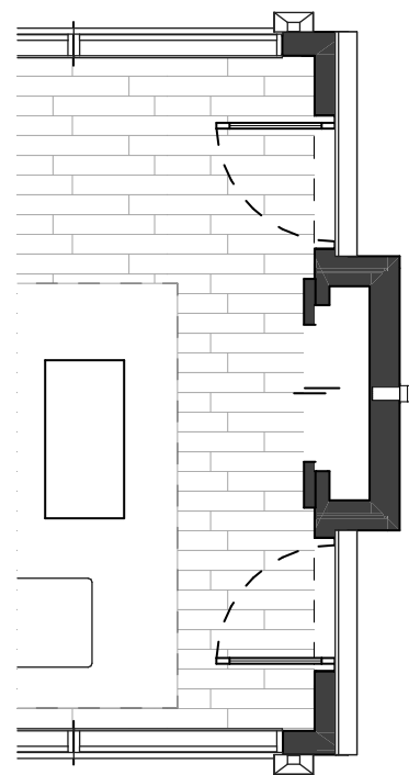
1 GARAGE PLAN 3/16" = 1'-0"
