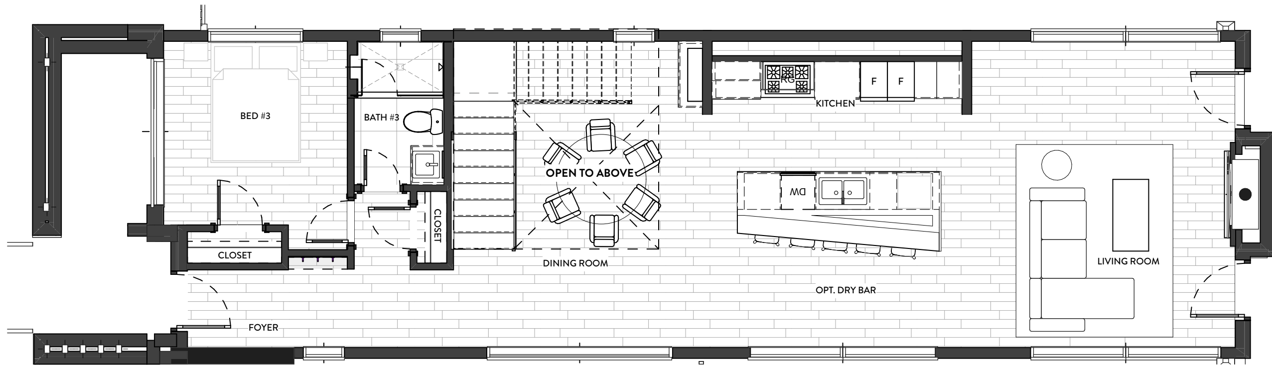
1 FIRST FLOOR PLAN 3/16" = 1'-0"
